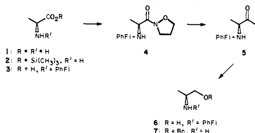
Scheme II
